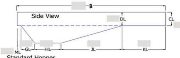
Standard Hopper With Safety Ledge
